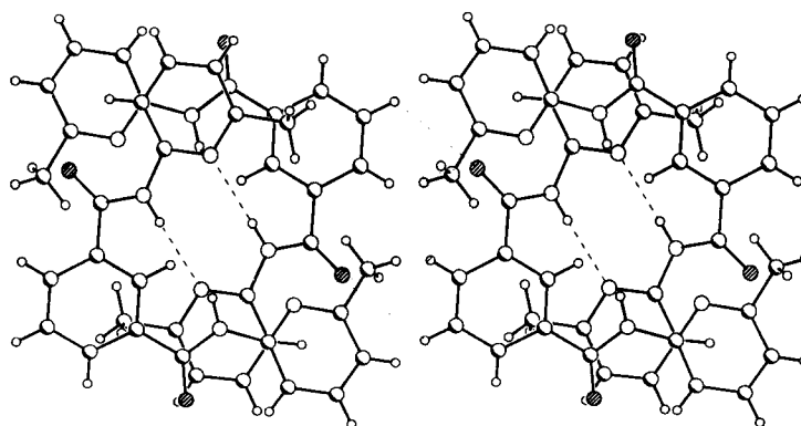
Figure 3. Packing of 1 in the crystal (view down the axis b).
