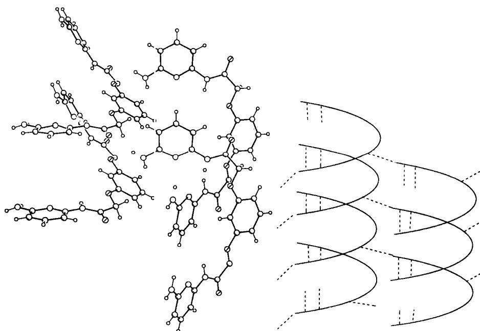
Figure 6. X-ray and schematic structure of the packing of 4 .
