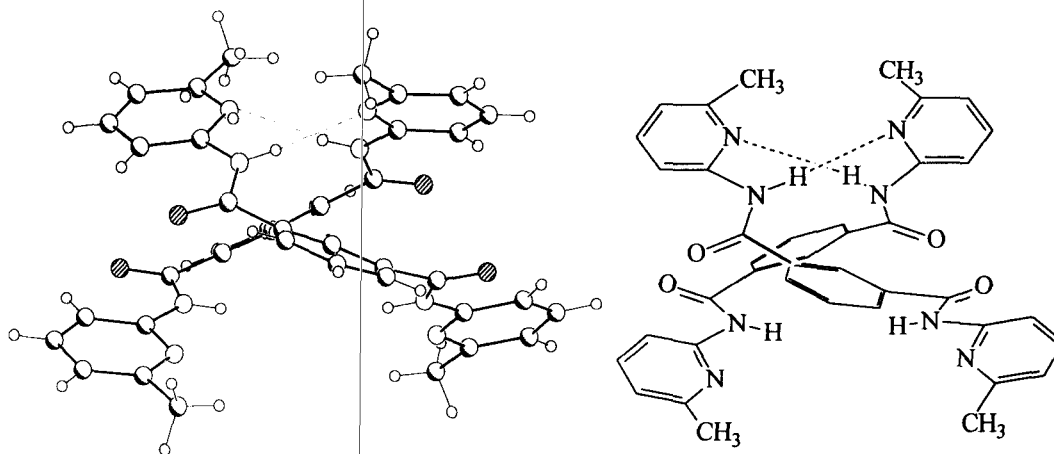
Figure 2. X-ray and schematic structure of the dimer of 1 .
