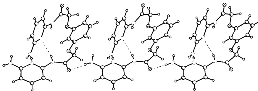
Figure 7. X-ray structure of the packing of 4 (view down the axis b)
